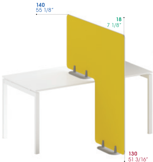
Con supporti in Zama / With Zamac clamps
