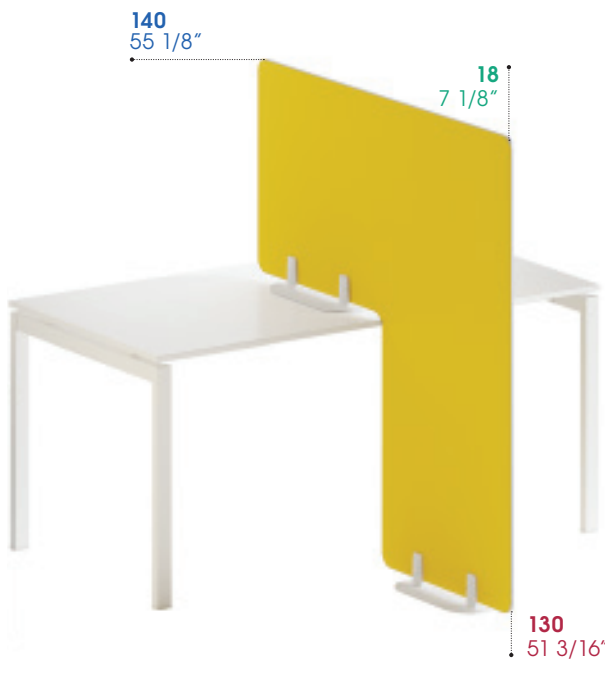
Con supporti in ABS / With ABS clamps
